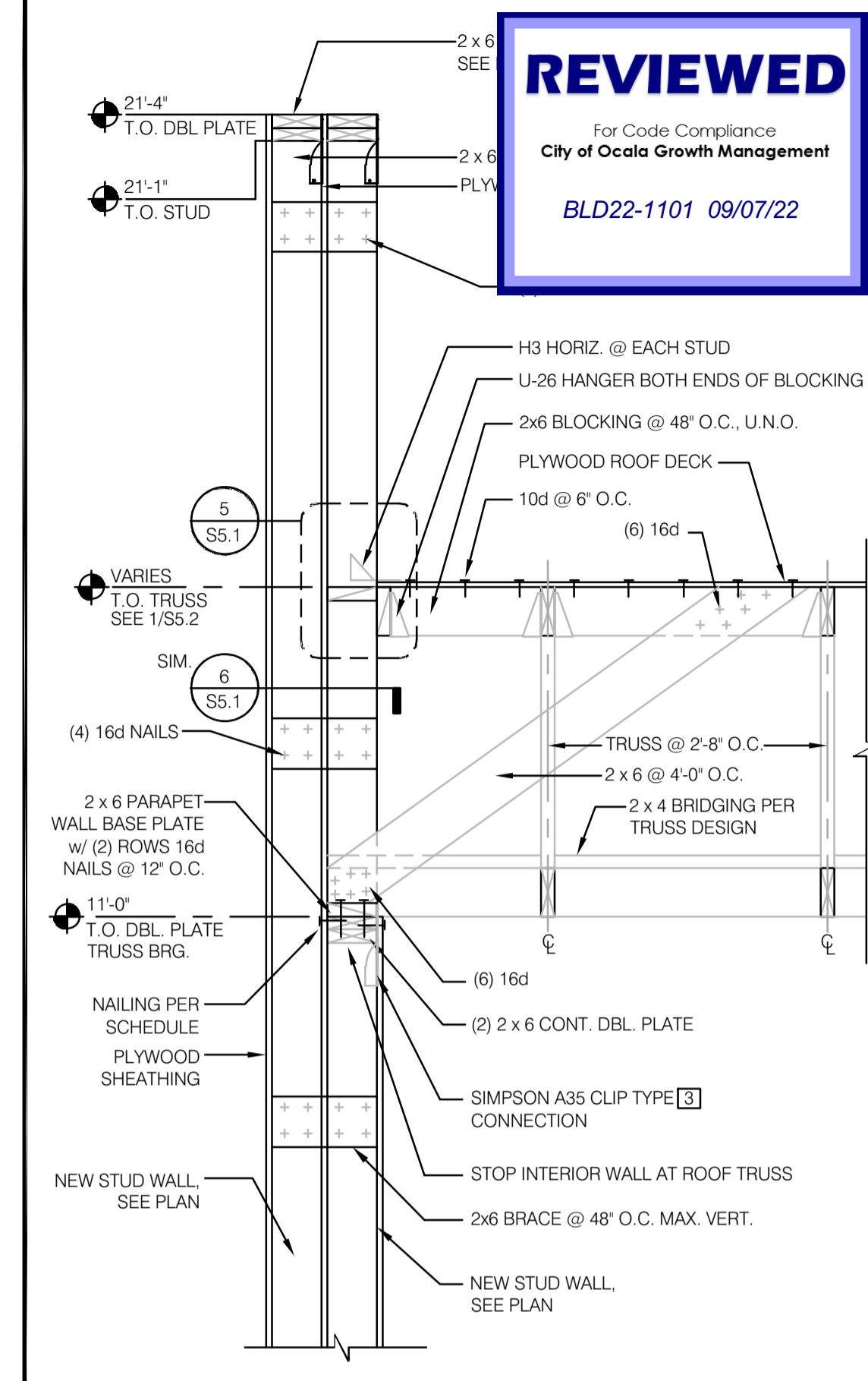
TOWER FRONT WALL @ TRUSS 3/4" = 1'-0" 2
