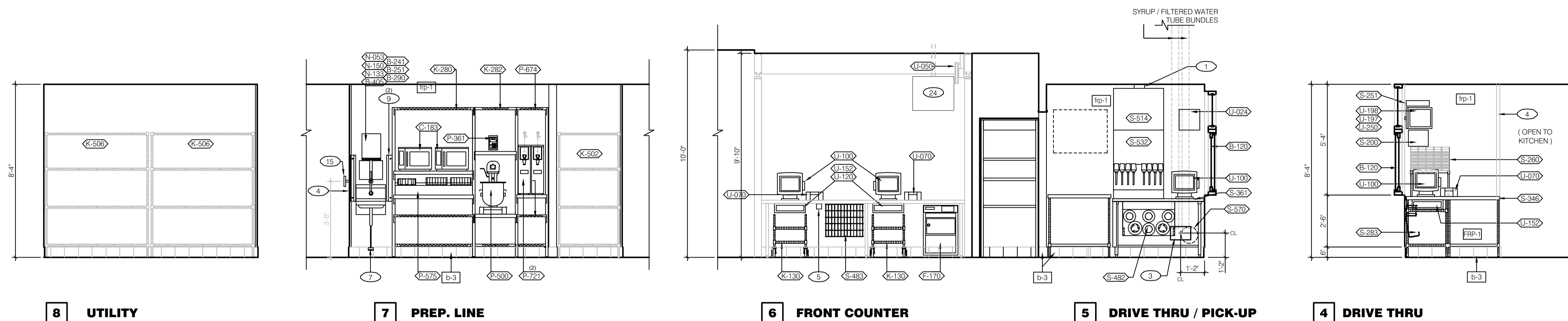
KITCHEN ELEVATIONS 3/8" = 1'-0"
