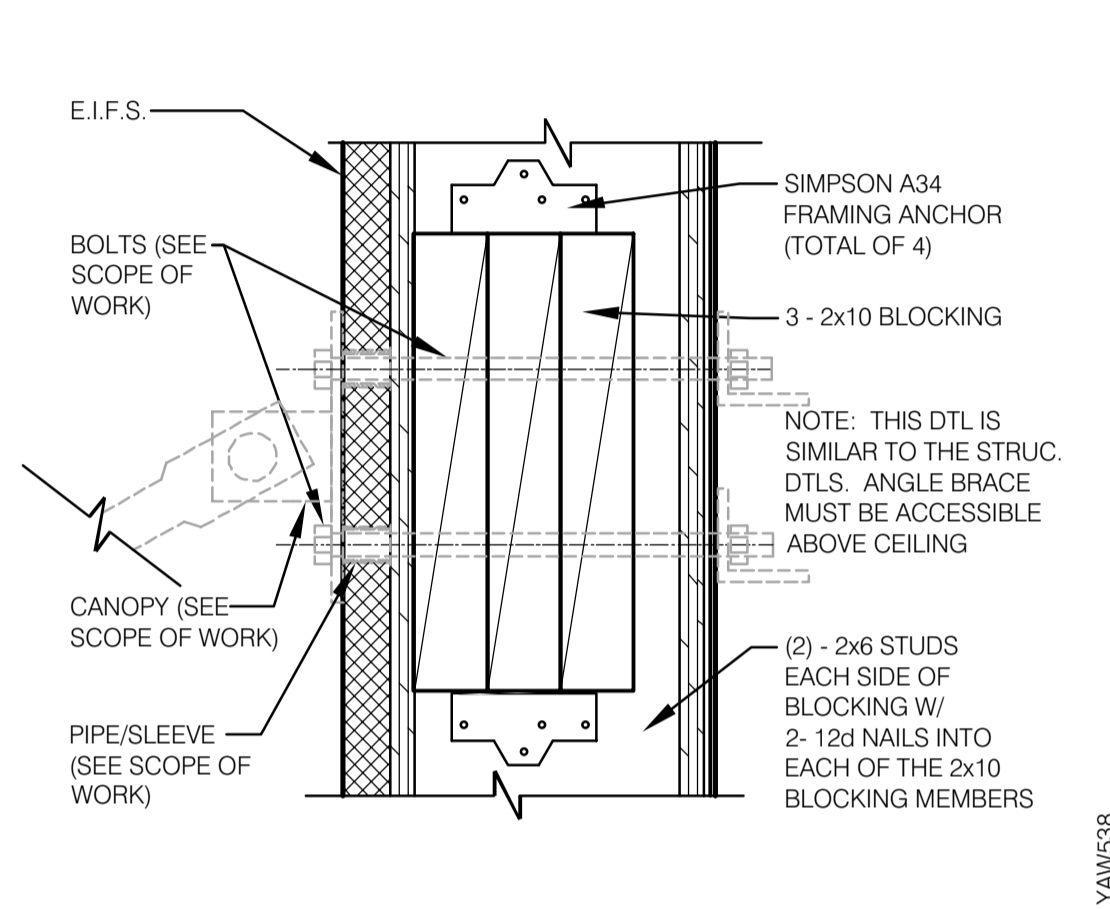
CANOPY TIE-ROD BLOCKING DETAIL 3' = 1'-0" 6
