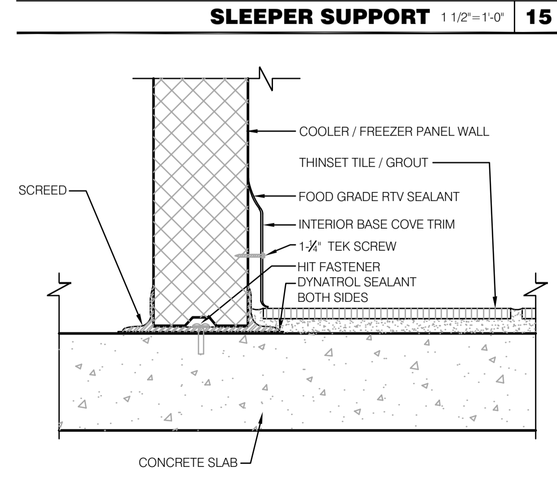
TILE/BASE at COOLER/FREEZER 3' = 1'-0" 16
