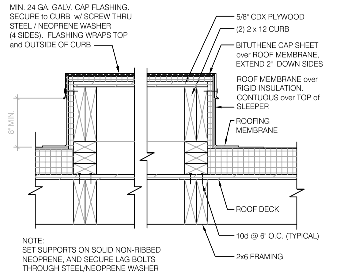
SLEEPER SUPPORT 1 1/2' = 1'-0" 15
