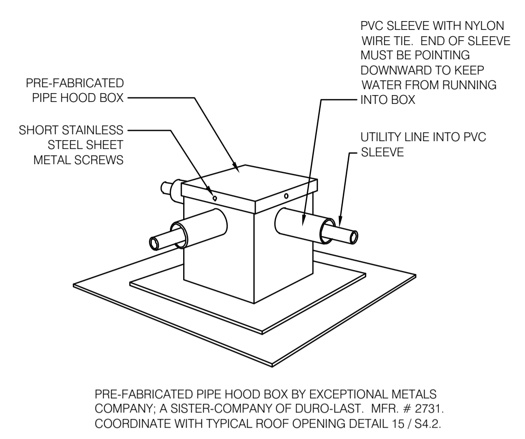
PIPE HOOD DETAIL NTS 9
