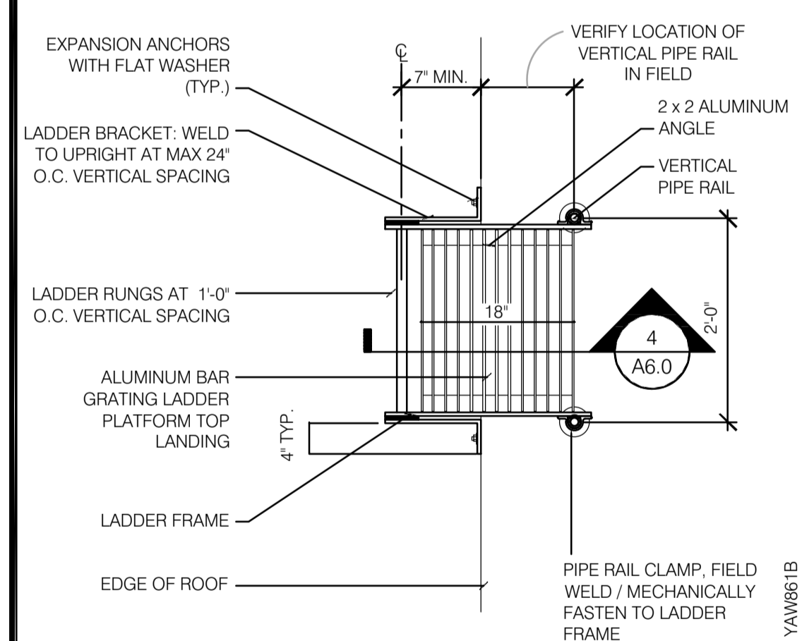
ROOF LADDER 1' = 1'-0" 19
