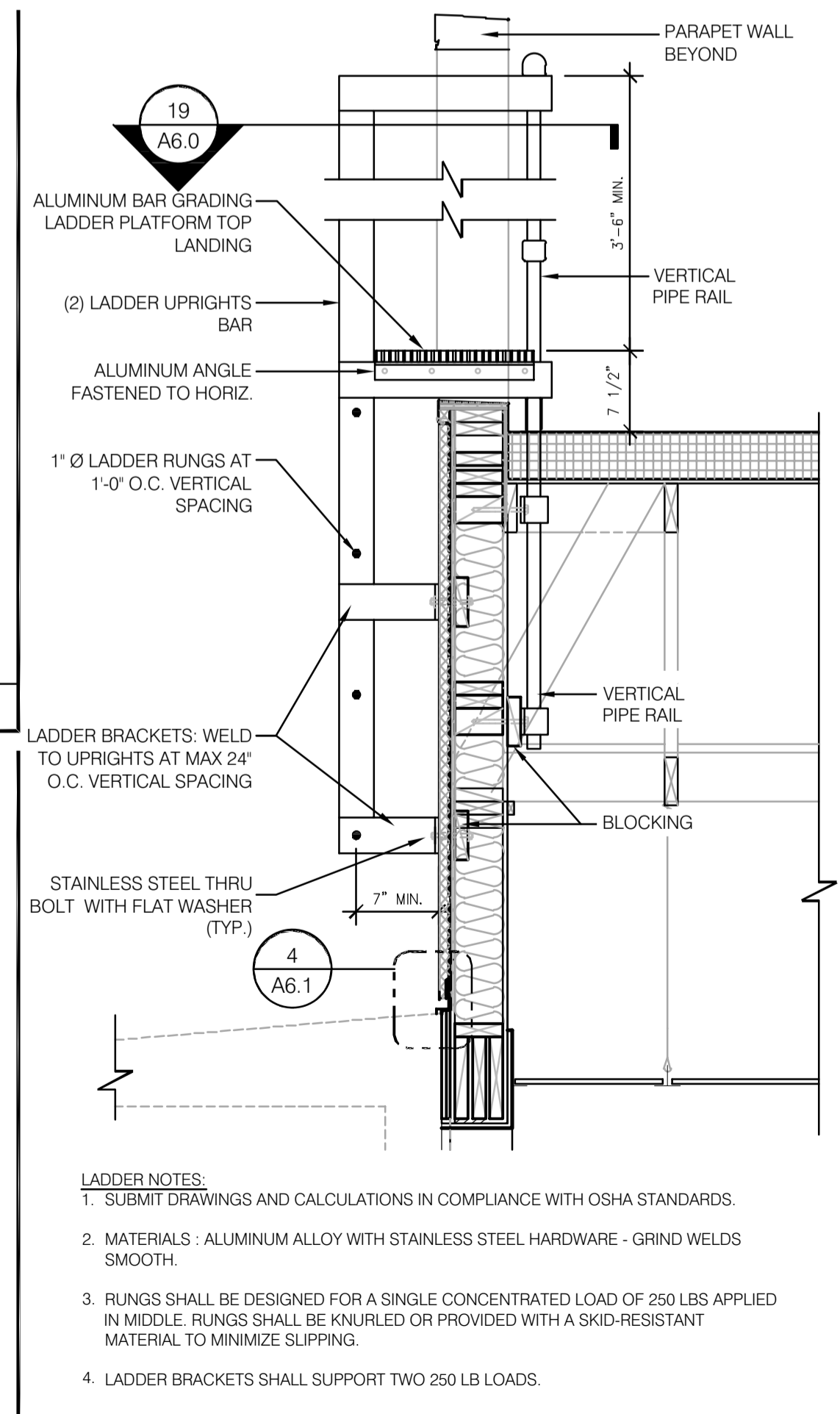
ROOF LADDER 1' = 1'-0" 4
