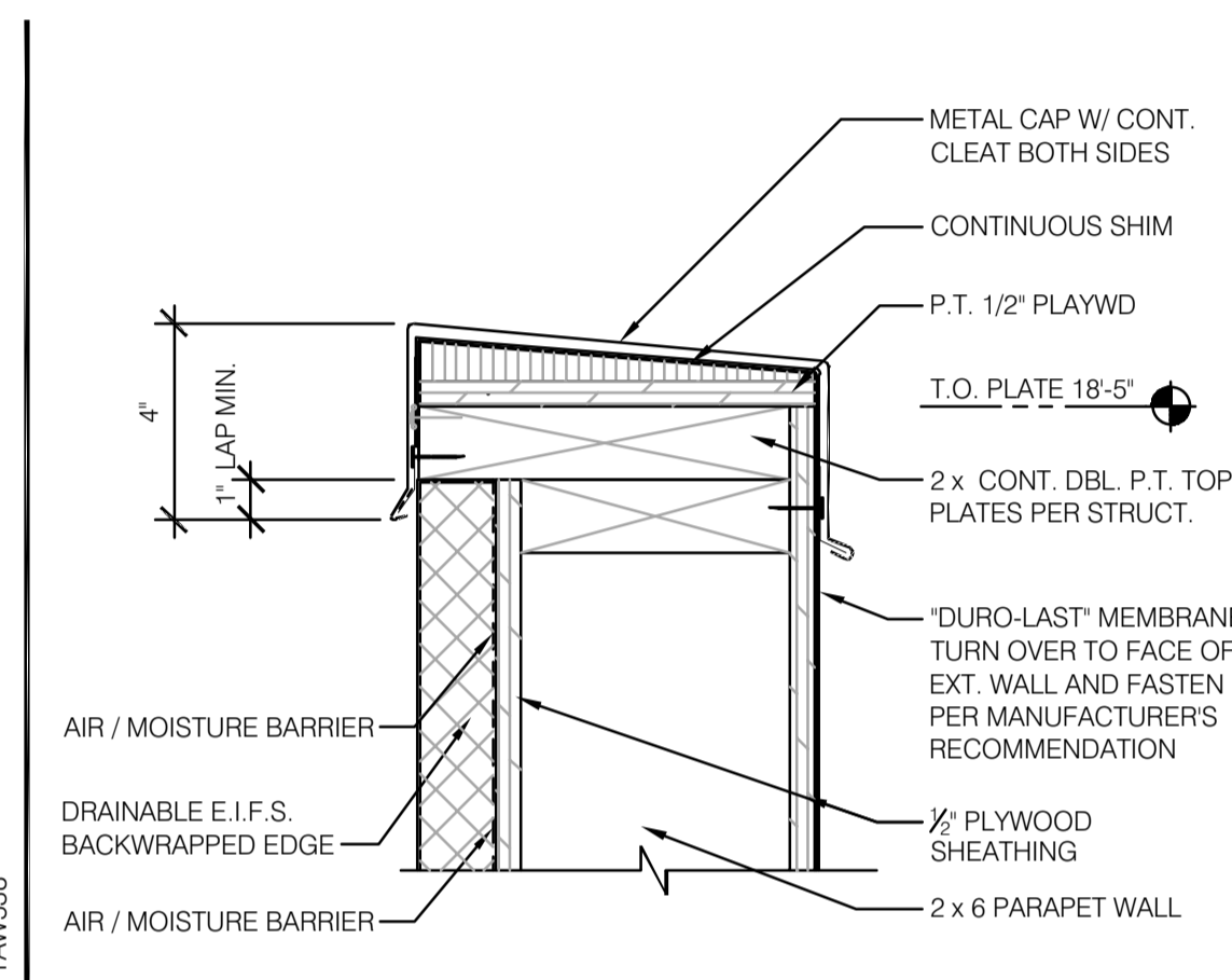
PARAPET COPING TYPICAL 3' = 1'-0" 2
