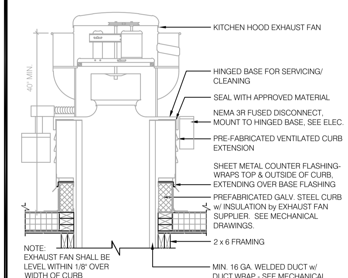
CURB for EXHAUST FANS EF-1 / EF-2 N.T.S. 18
