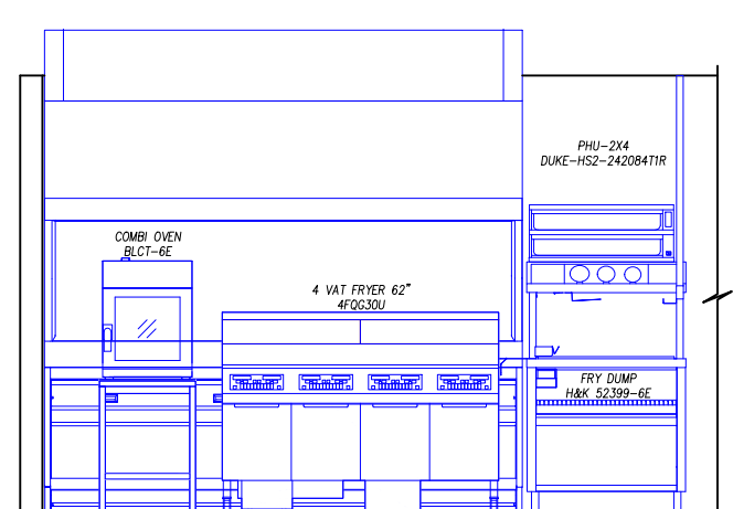
H FRYER HOOD ELEVATION
