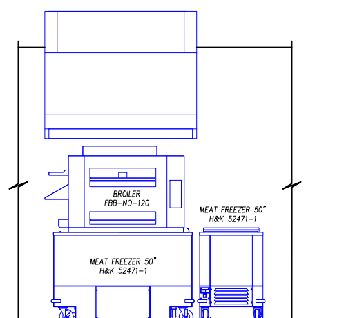
J BROILER HOOD ELEVATION
