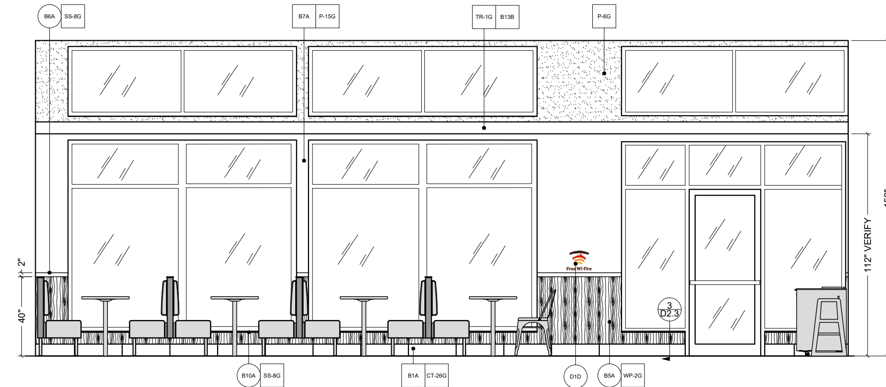
E ELEVATION 1/4" = 1'-0"
