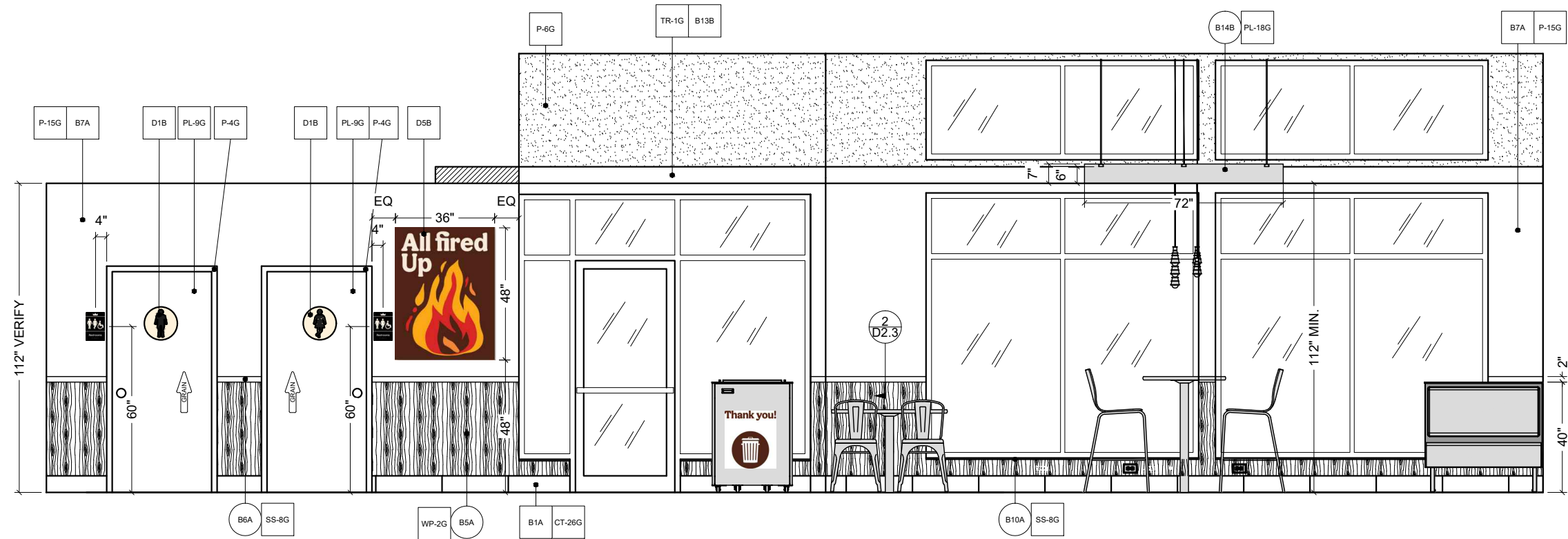
D ELEVATION 1/4" = 1'-0"
