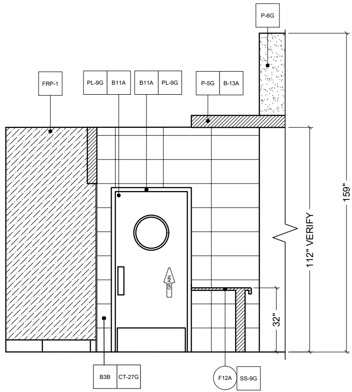
B ELEVATION 1/4" = 1'-0"
