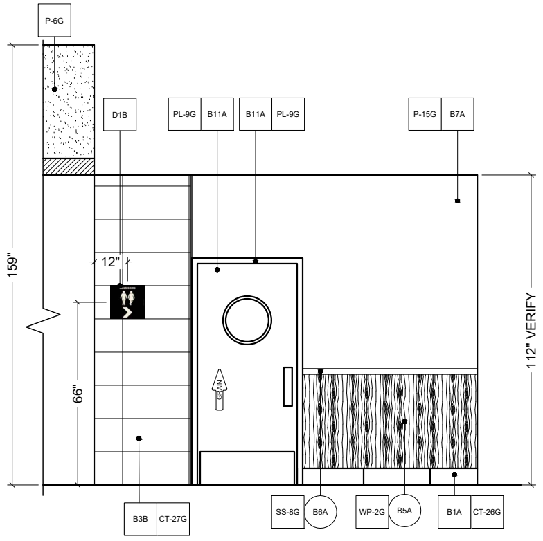
C ELEVATION 1/4" = 1'-0"
