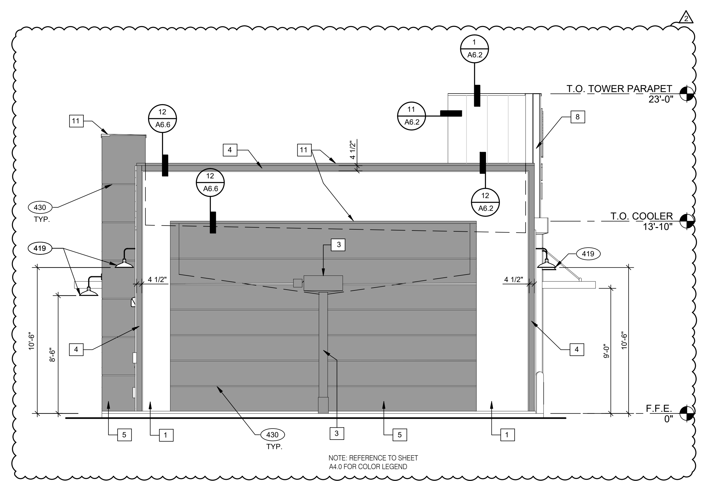
WEST ELEVATION 1/4" = 1'-0" 3
