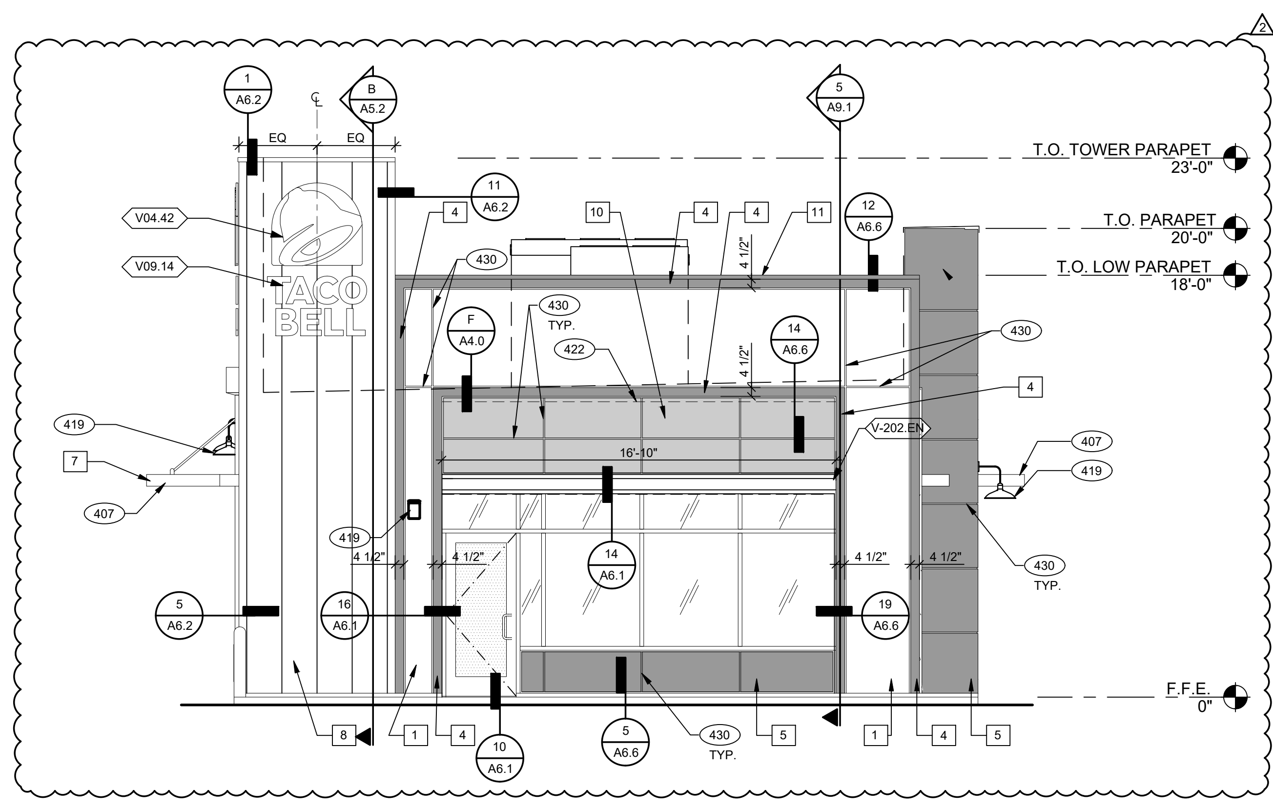
EAST ELEVATION 1/4" = 1'-0" 2
