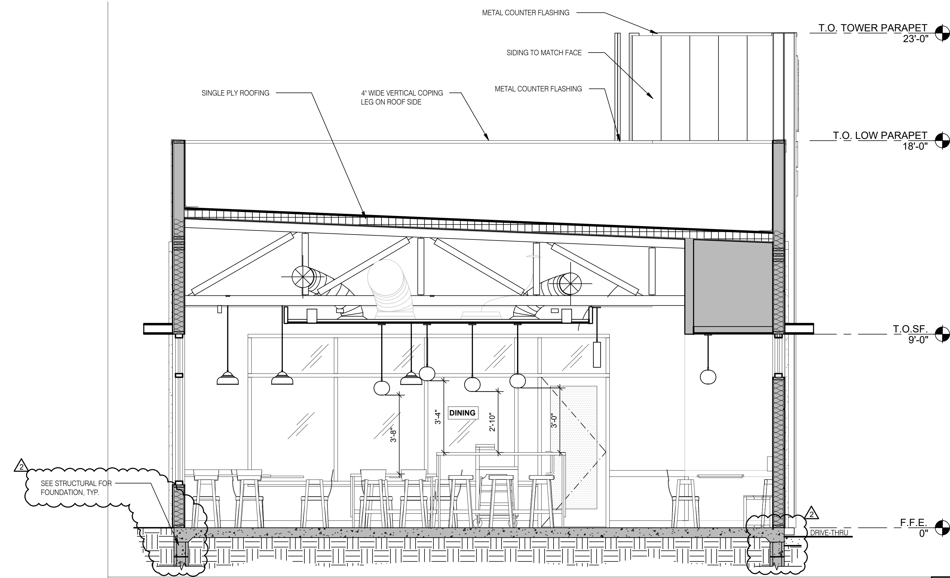
BUILDING SECTION 5 3/8" = 1'-0" A
