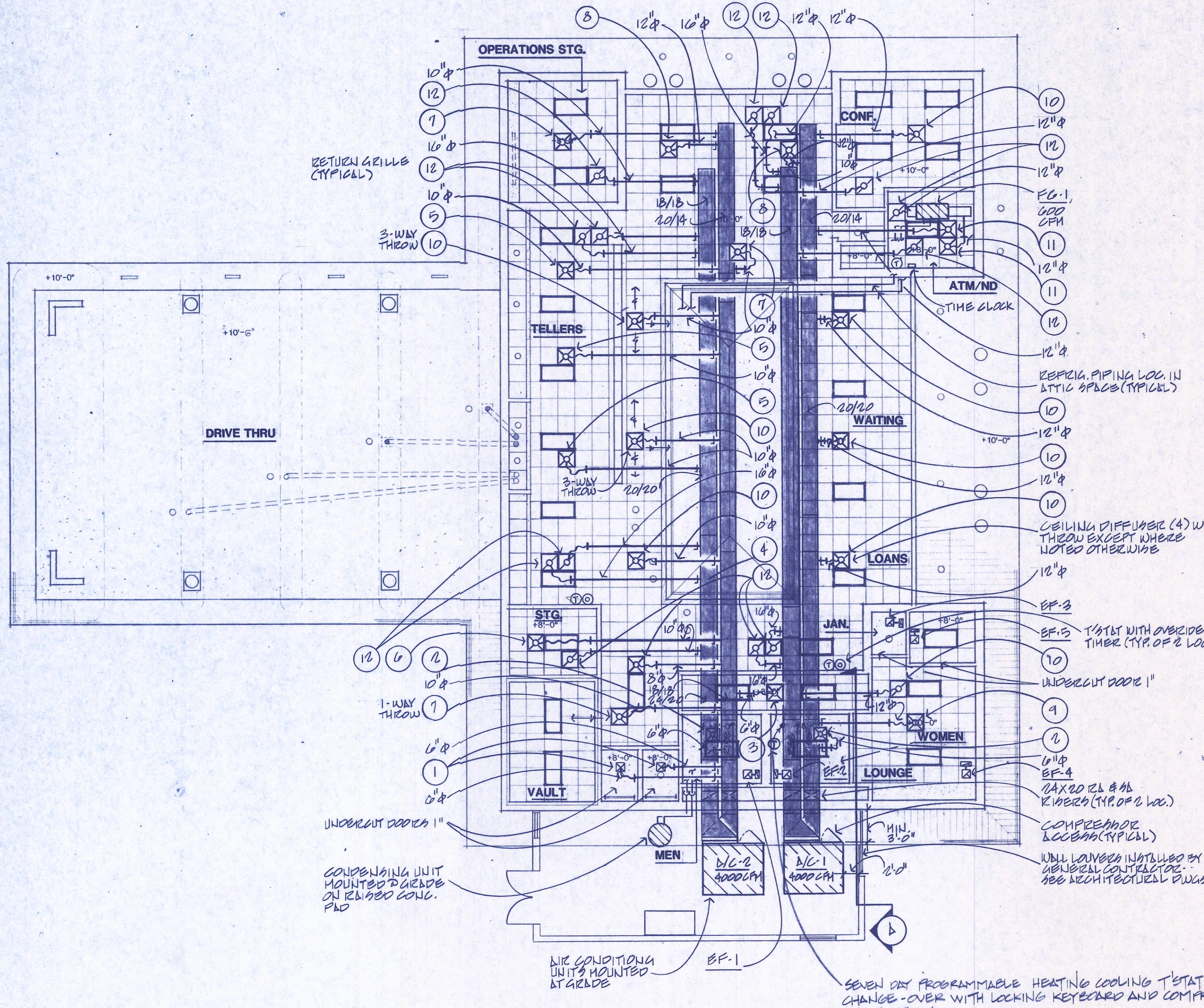
MECHANICAL FLOOR PLAN SCALE 1/8"=1'-0"
