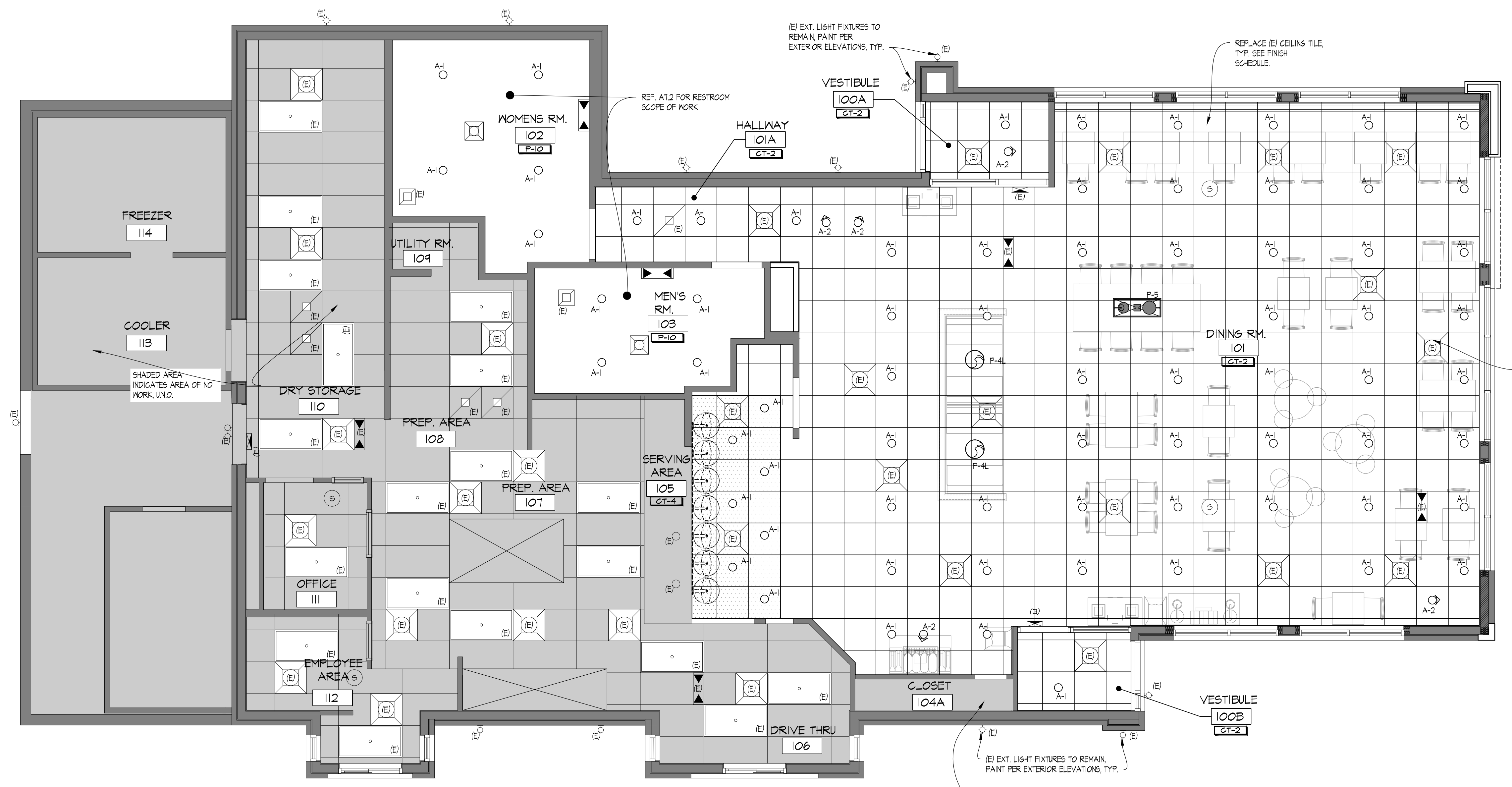
01 REFLECTED CEILING PLAN SCALE: 1/4" = 1'-0"
