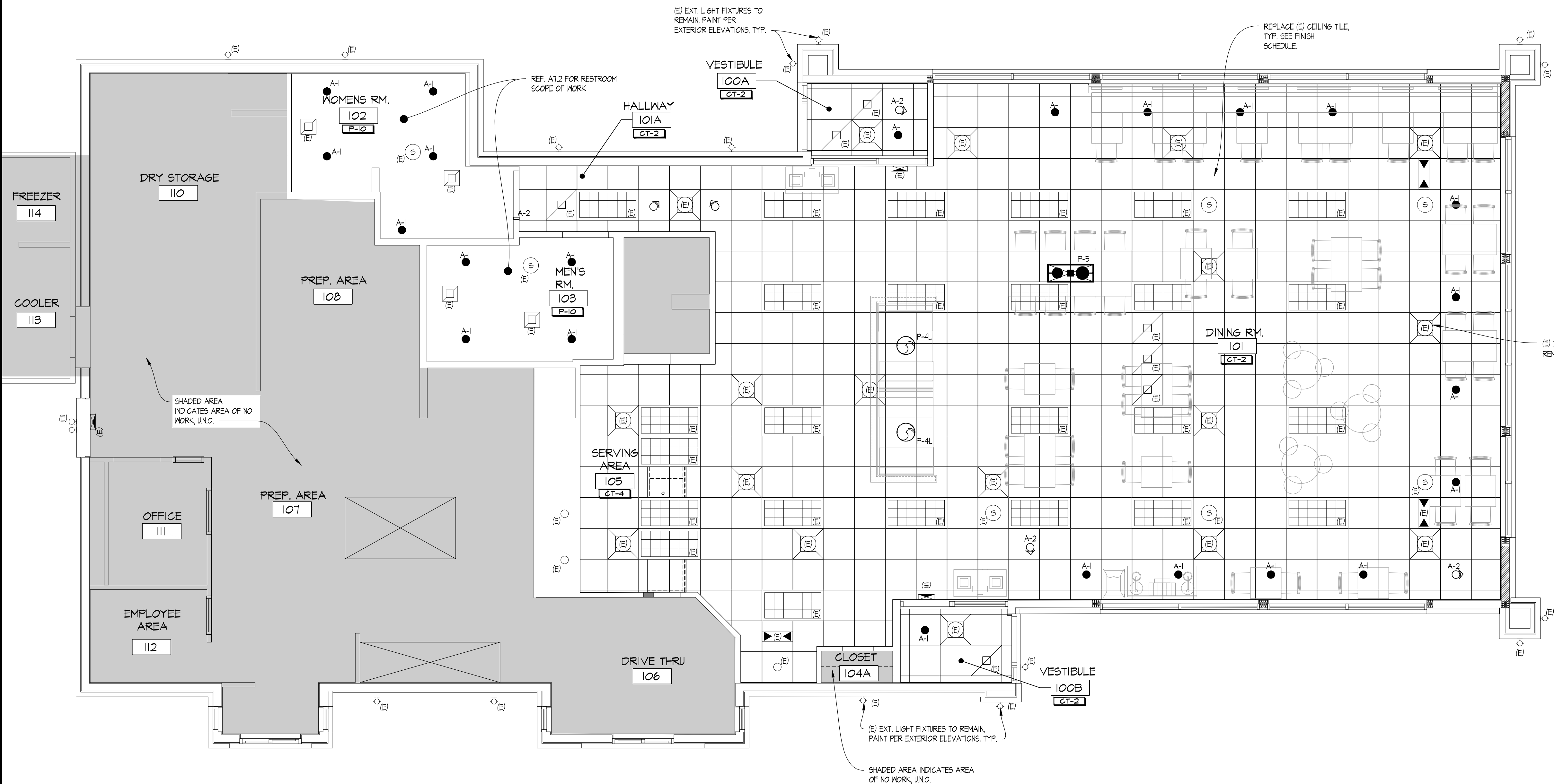
01 REFLECTED CEILING PLAN SCALE: 1/4" = 1'-0"
