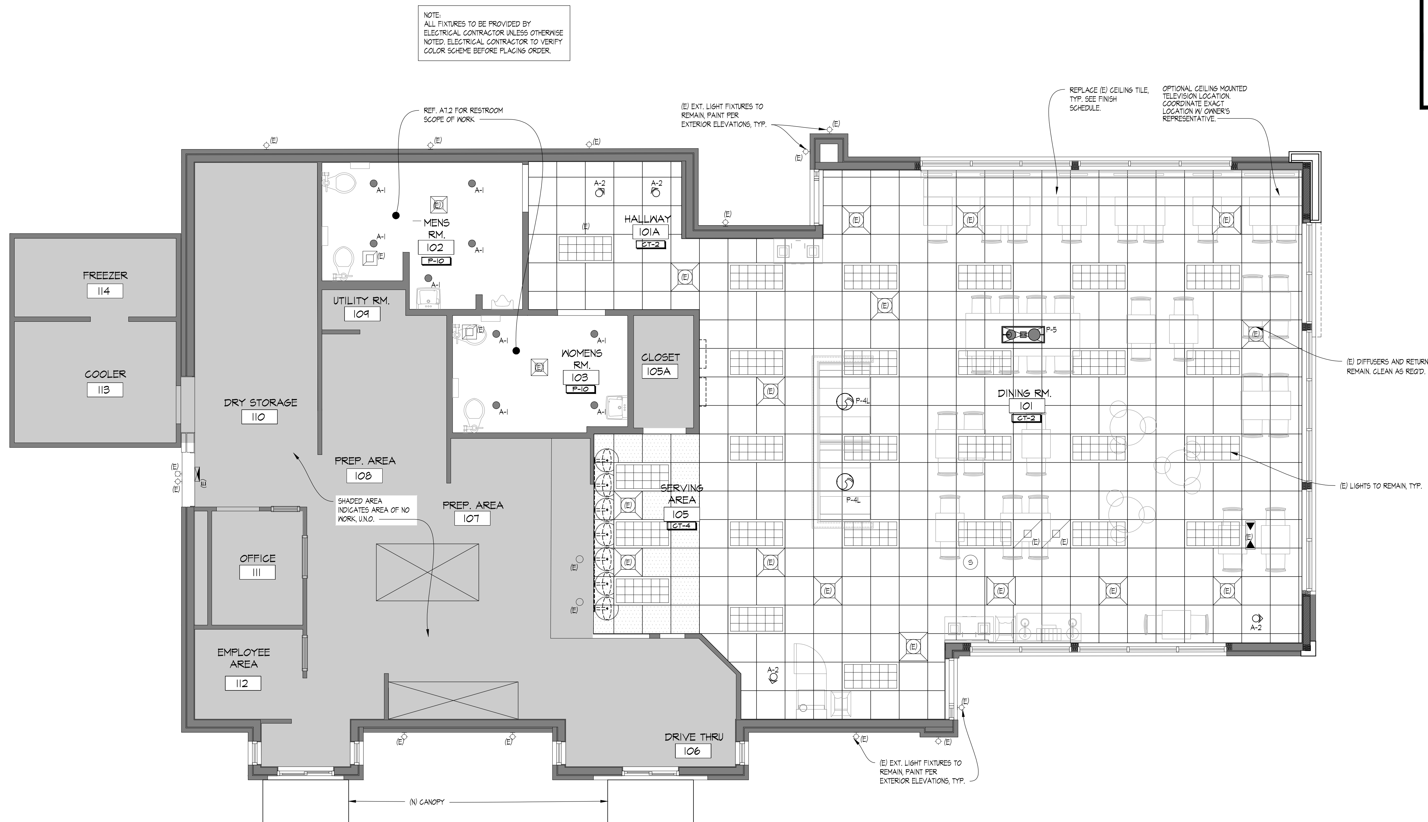
01 REFLECTED CEILING PLAN SCALE: 1/4" = 1'-0"
