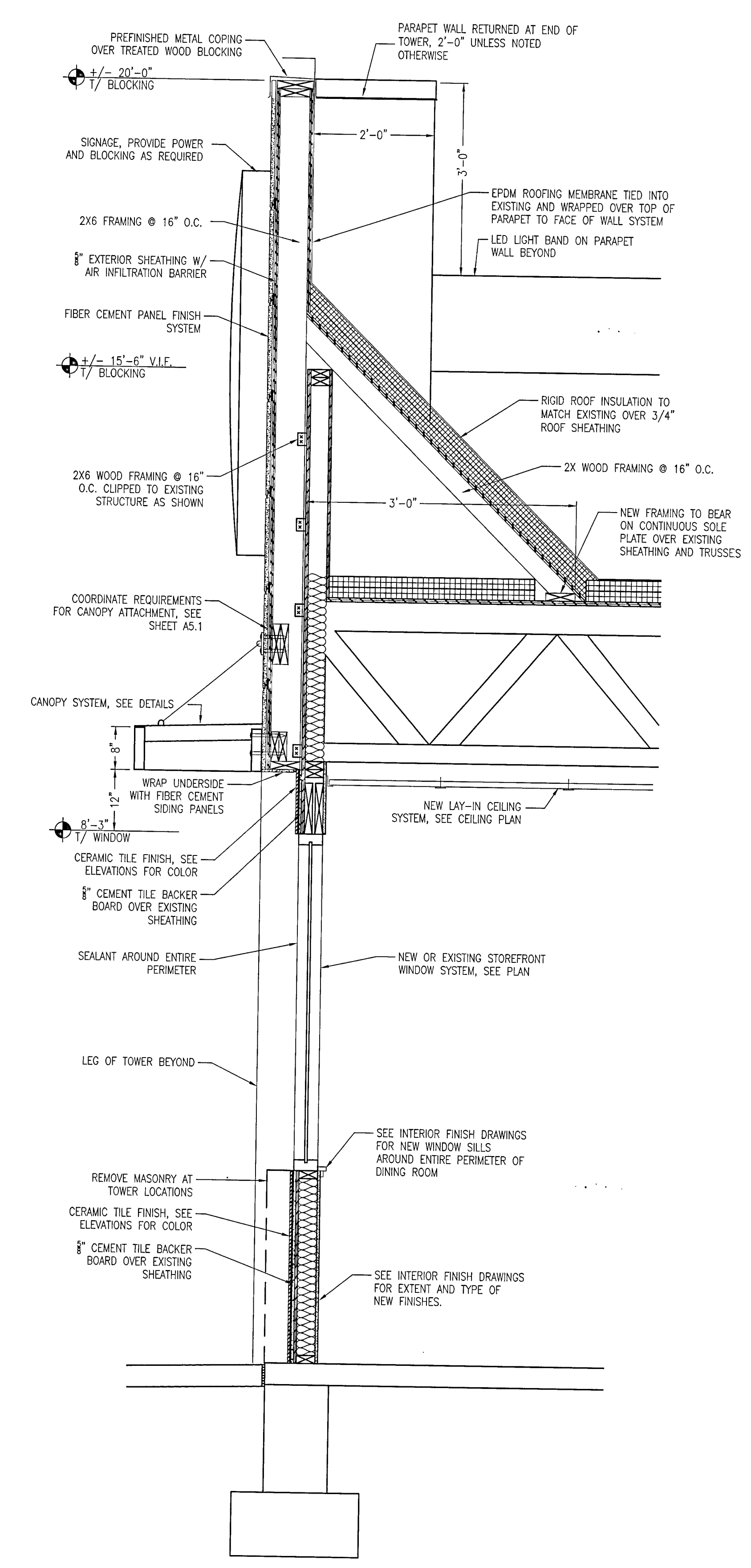
SECTION @ TOWER WINDOW 1 3/4" = 1'-0"
