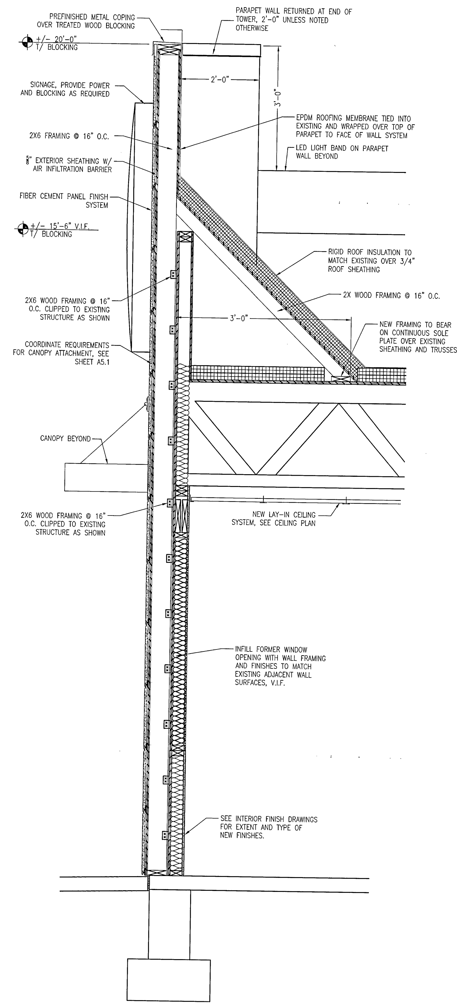
SECTION @ TOWER LEG 2 3/4" = 1'-0"
