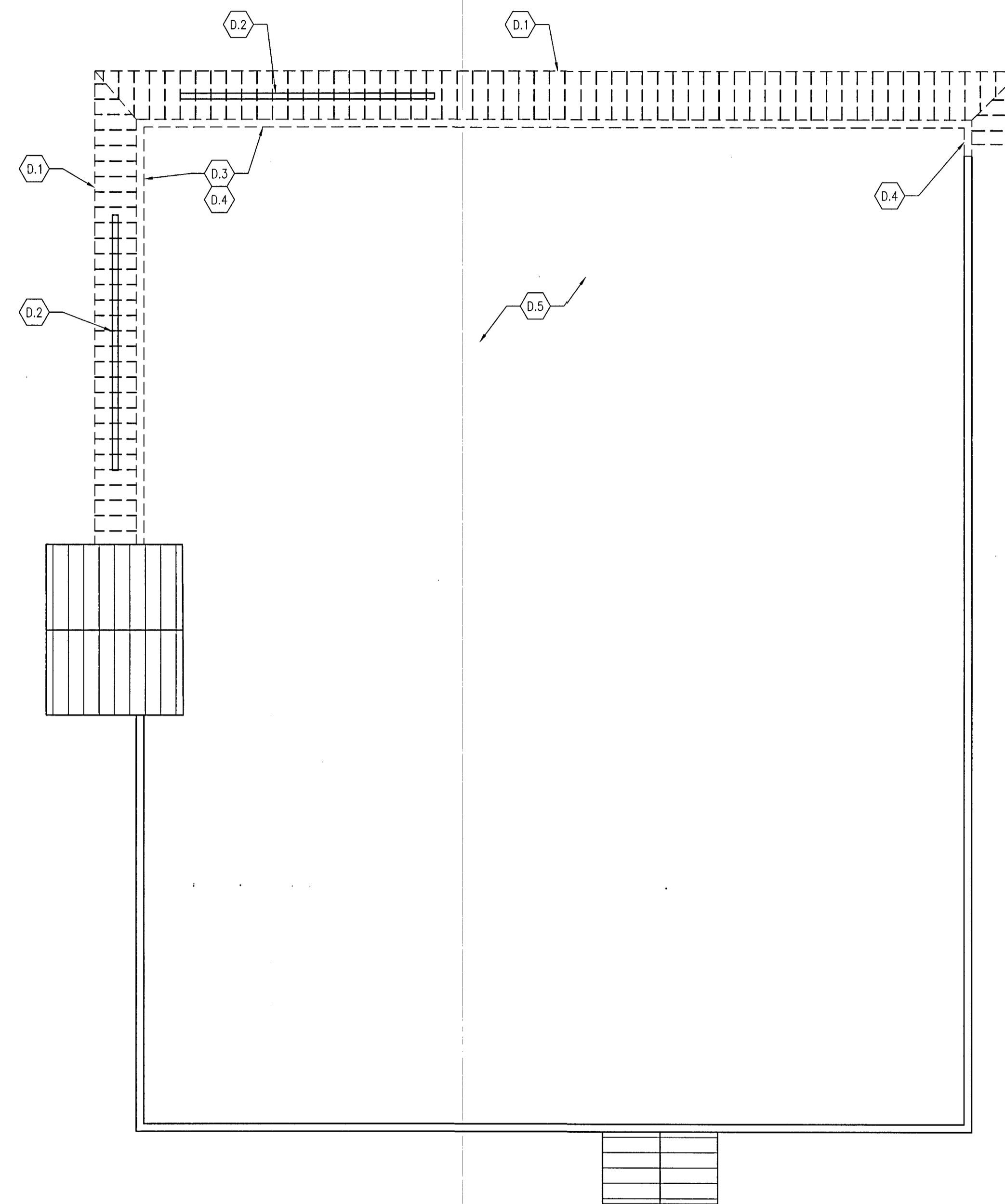
DEMOLITION ROOF PLAN 1/8" = 1'-0"
