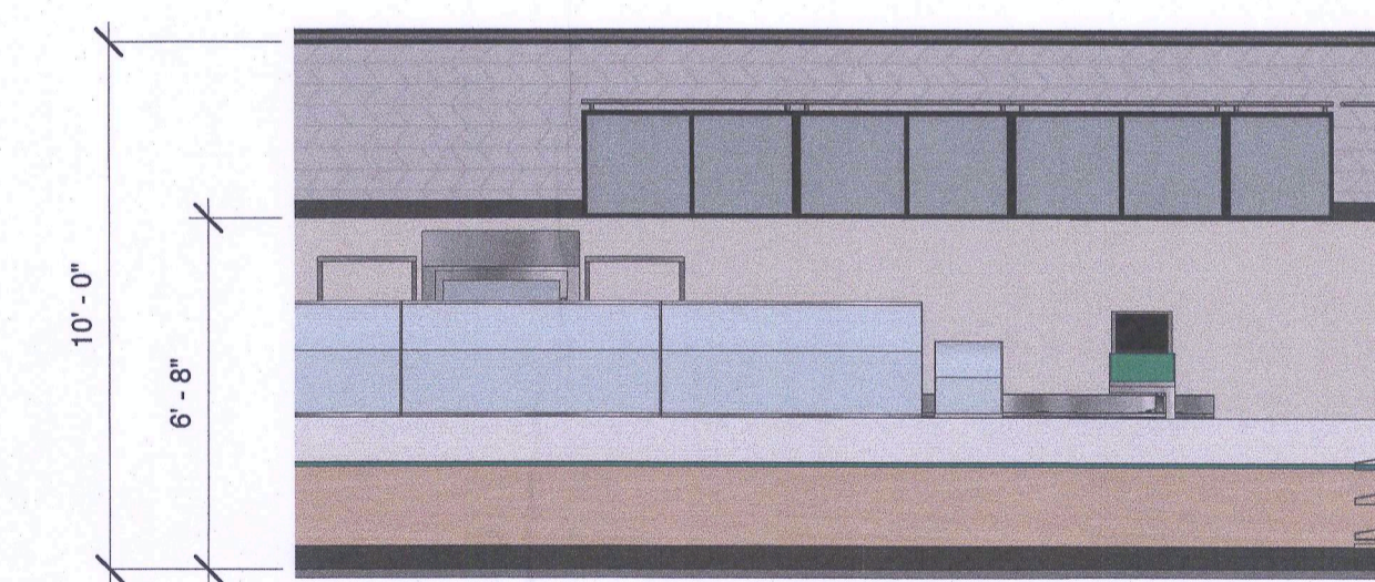
3 Service Area Elevation 1/4" = 1'-0"
