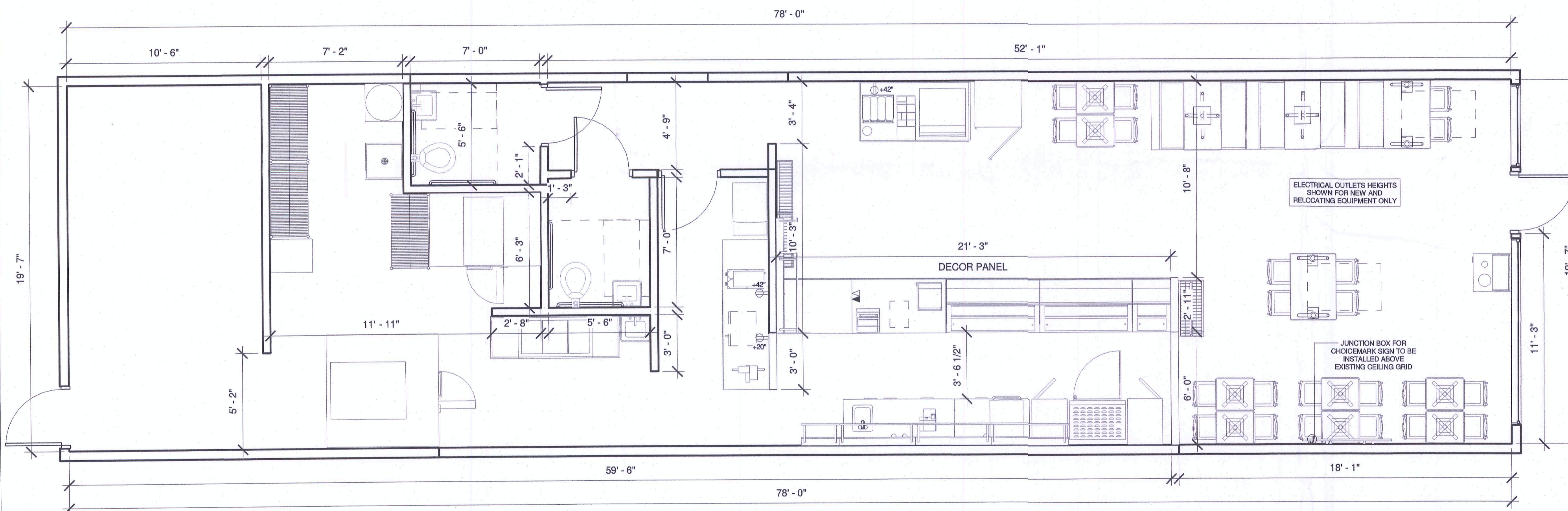
2 DIMENSION & ELECTRICAL PLAN 1/4" = 1'-0"
