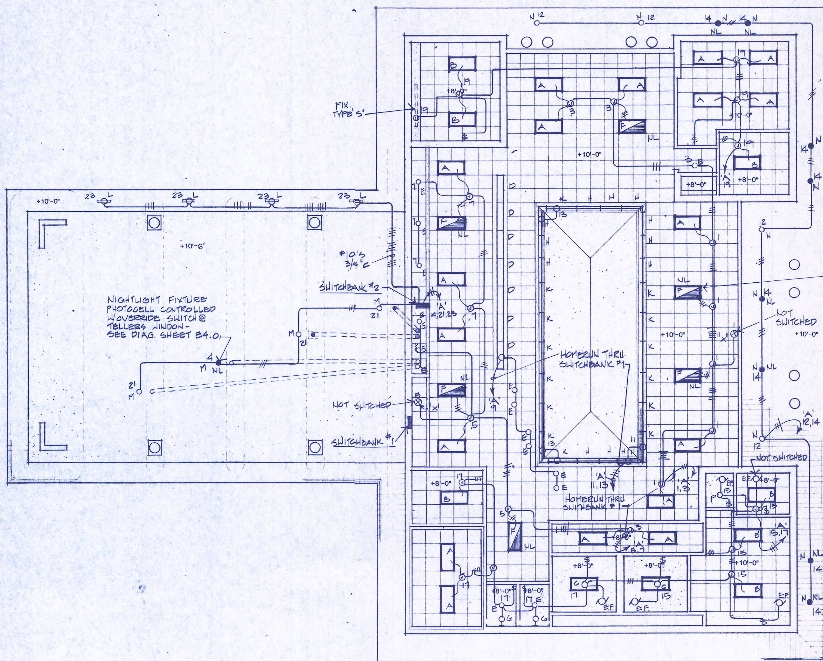
ELECTRICAL LIGHTING PLAN 1/8"=1'-0"
