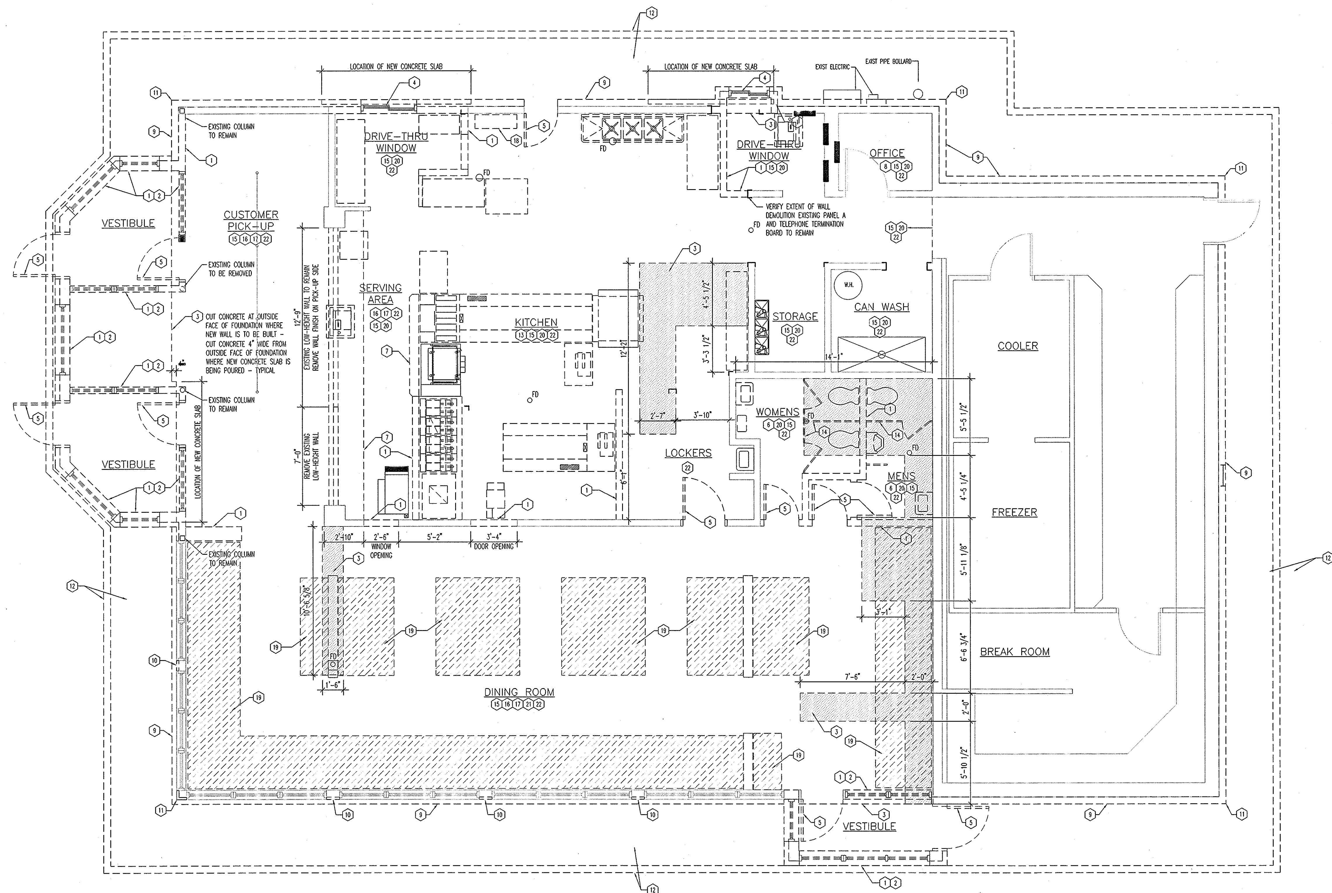
1 DEMOLITION PLAN SCALE: 1/4"=1'-0"
