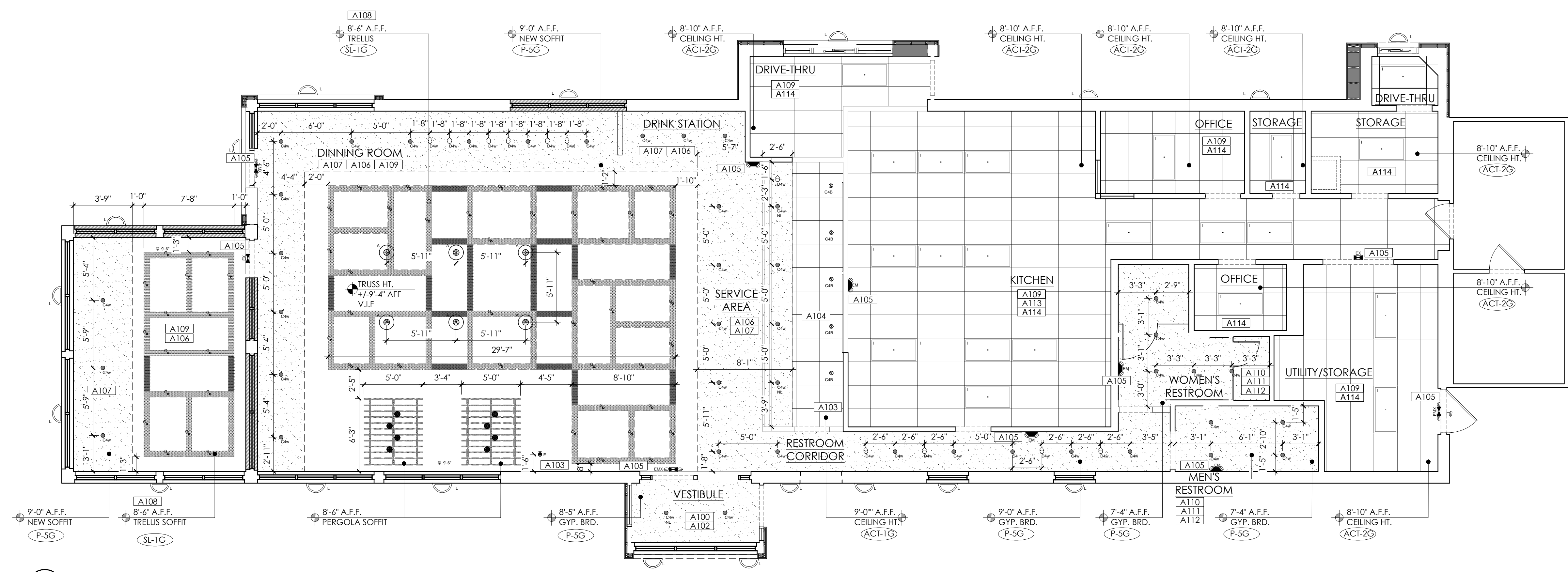
1 PROPOSED REFLECTED CEILING PLAN SCALE: 3/16" = 1'-0"
