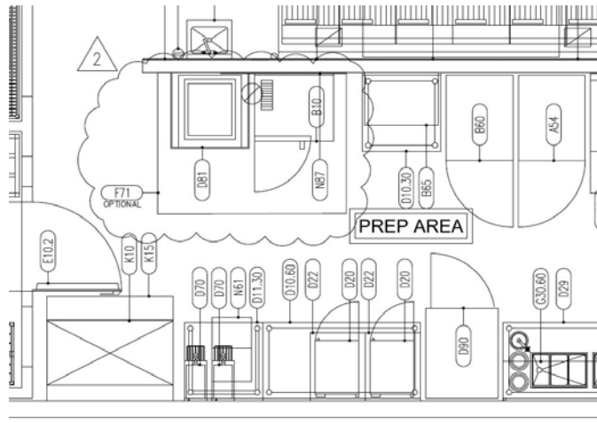
1 EQUIPMENT PLAN K1 1/4"=1'-0"
