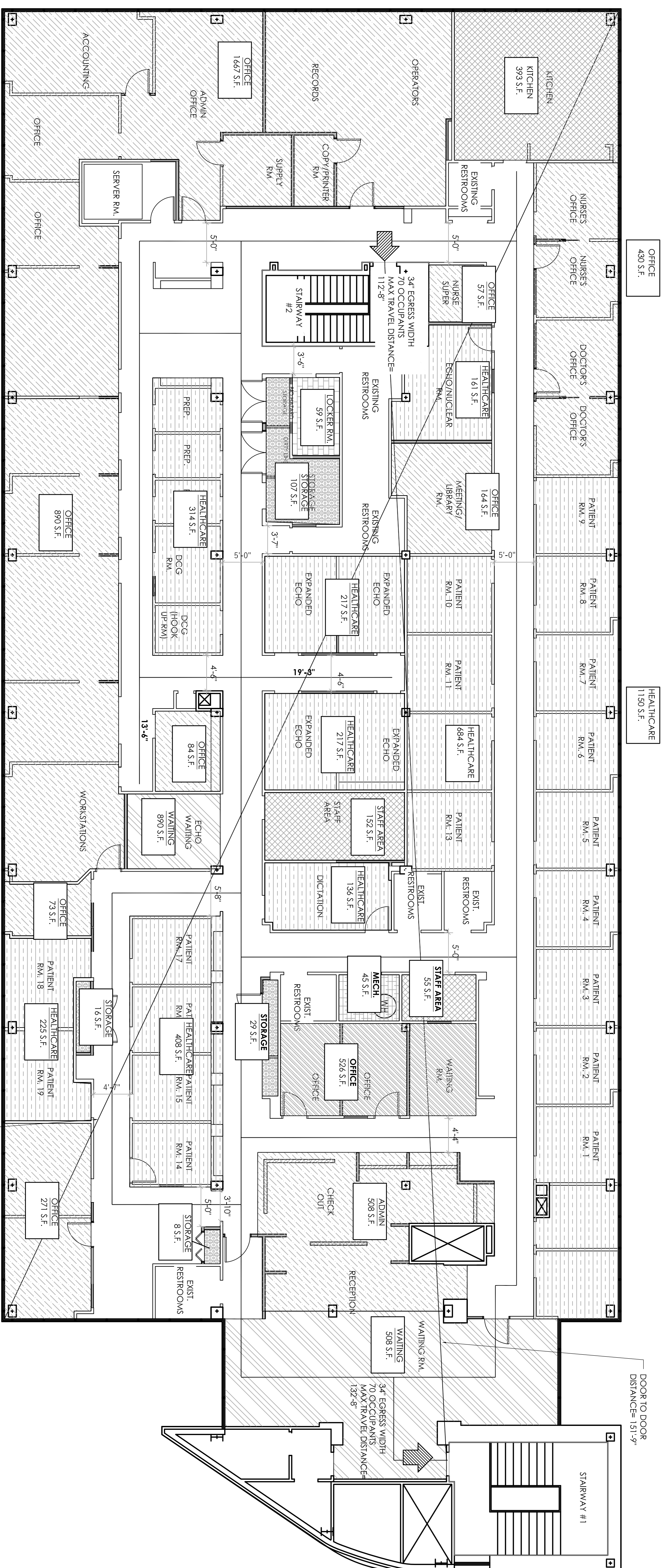
1 LIFE SAFETY PLAN SCALE: 1/8" = 1'-0"
