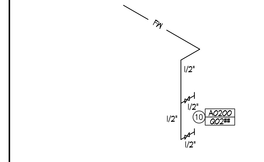
PARTIAL WATER SUPPLY ISOMETRIC NO SCALE
