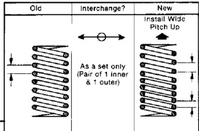
Ref. Nos. 3 & 4, Valve Springs
