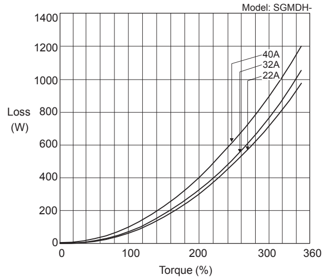
SGMDH Servomotors
