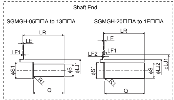
Note: For the specifications of the other shaft ends, refer to 3.19 Shaft End Specifications for SGMGH, SGMSh and SGMdH Servomotors.
