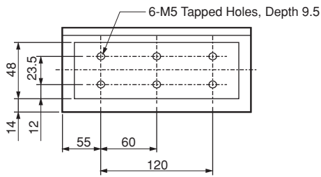
① SGLFW-50□200B□
