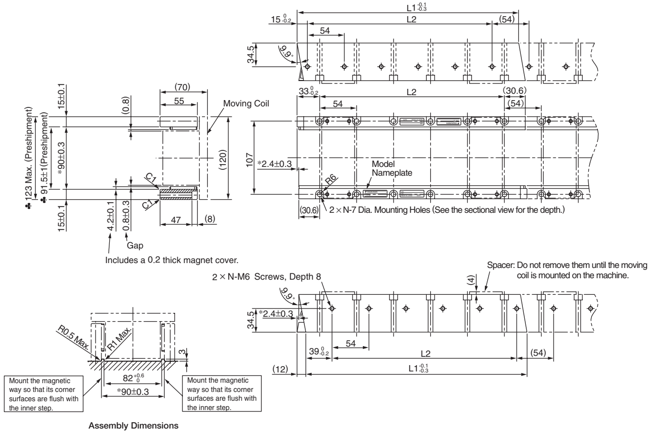
Assembly Dimensions
