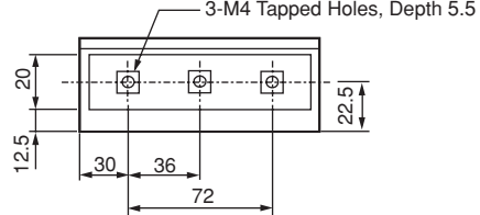
② SGLFW-20A120A□
