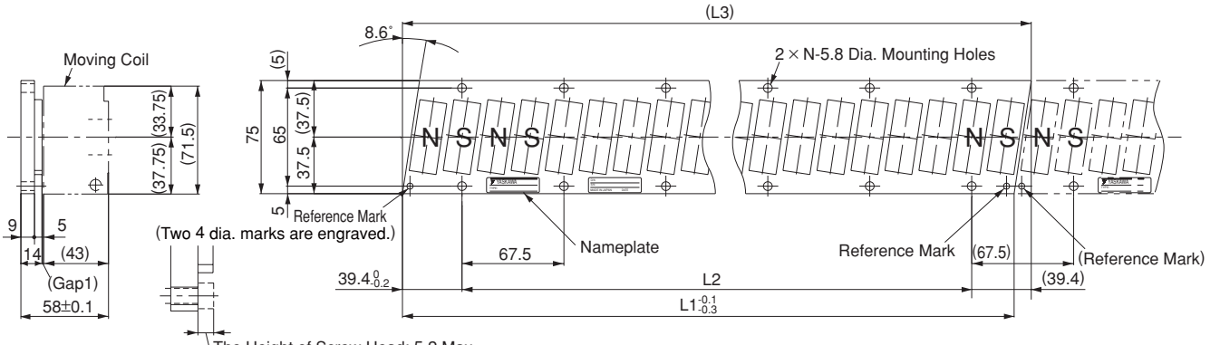
Assembly Dimensions
