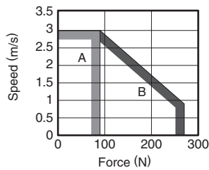
(1) SGTMF4A-027
