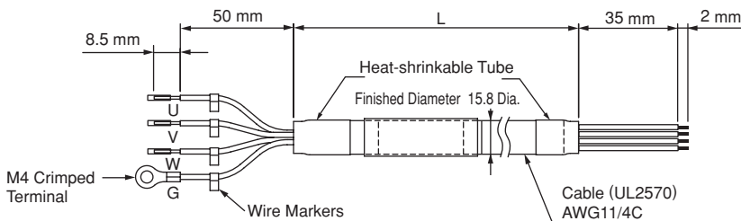
SERVOPACK-end Leads
