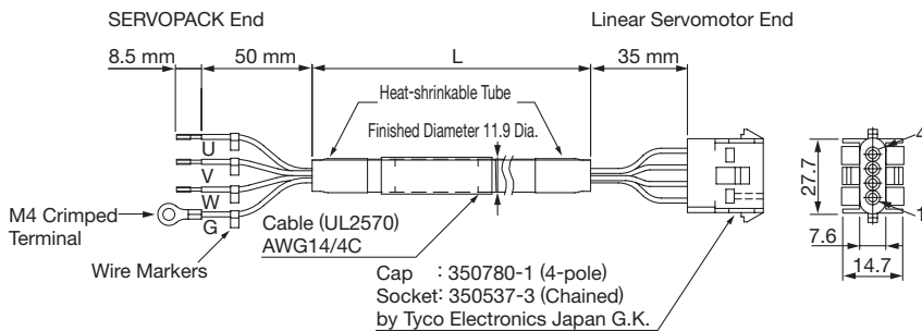
SERVOPACK-end Leads
