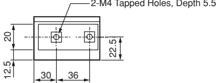
① SGLFW-20A090A□
