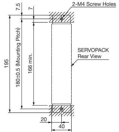
Mounting Hole Diagram
