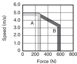
(1) SGT1F9□
