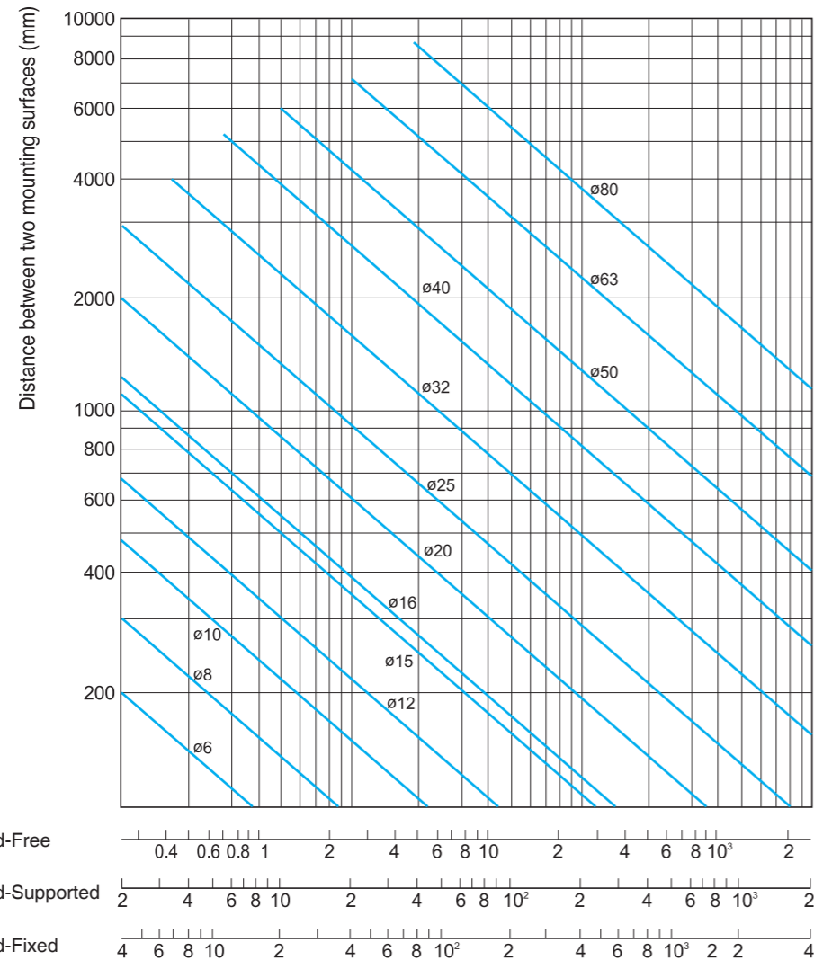
(Permissible tensile compressive load diagram)
