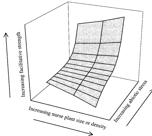
FIG. 1. Conceptual model of the effects of benefactor size, age, or density on the relative importance of positive and negative interactions on physical stress gradients. Under harsh physical conditions, increasing benefactor age, size, or density increases the relative strength of facilitation. Under benign physical conditions, increased benefactor age, size, or density increases the relative strength of the competitive effect.
